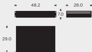
BeoSystem 4 with rack ears
