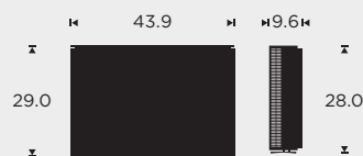
BeoSystem 4 with wall brackets
